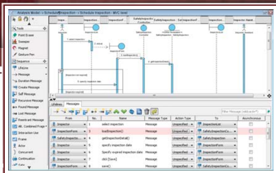
Sequence diagram with text editor
