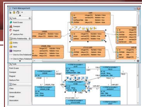
ERD and class diagram synchronization
