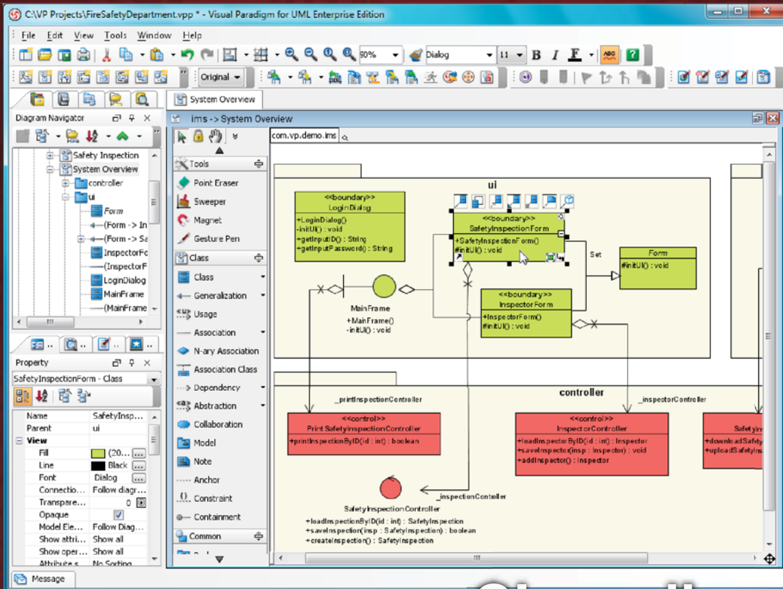
Class diagram
